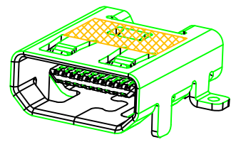
CONNECTOR 3D
